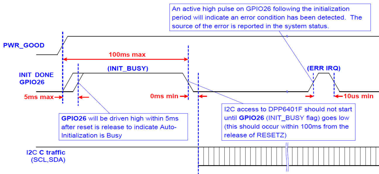
Figure 25. Internal Memory Test Diagram
