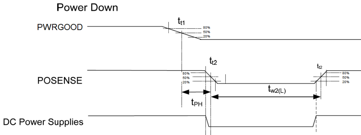
Figure 24. Power-Up/Down Timing
